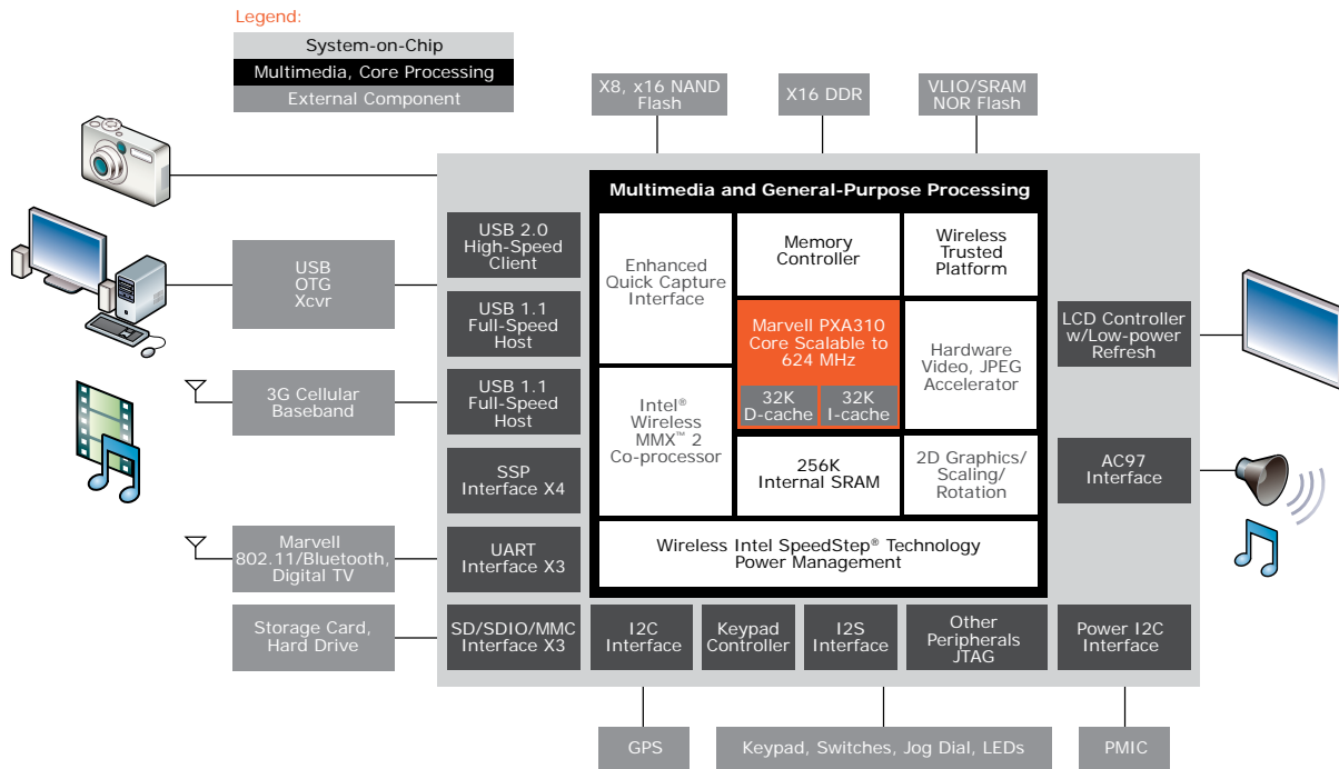
PXA310 System-on-Chip Block Diagram
